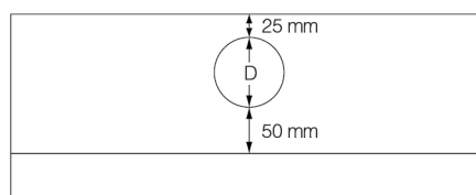
R-Round Inlet
