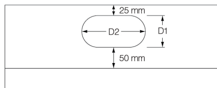
O-Oval Inlet
